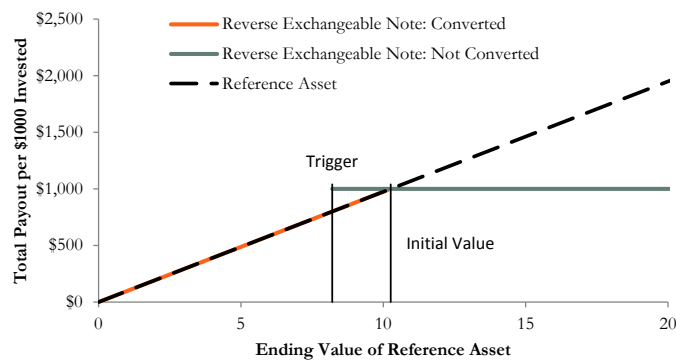
The payoff diagram shows the final payoff of this note given ION Geophysical Corporation's stock price (horizontal axis). For comparison, the dashed line shows the payoff if you invested in ION Geophysical Corporation's stock directly.
